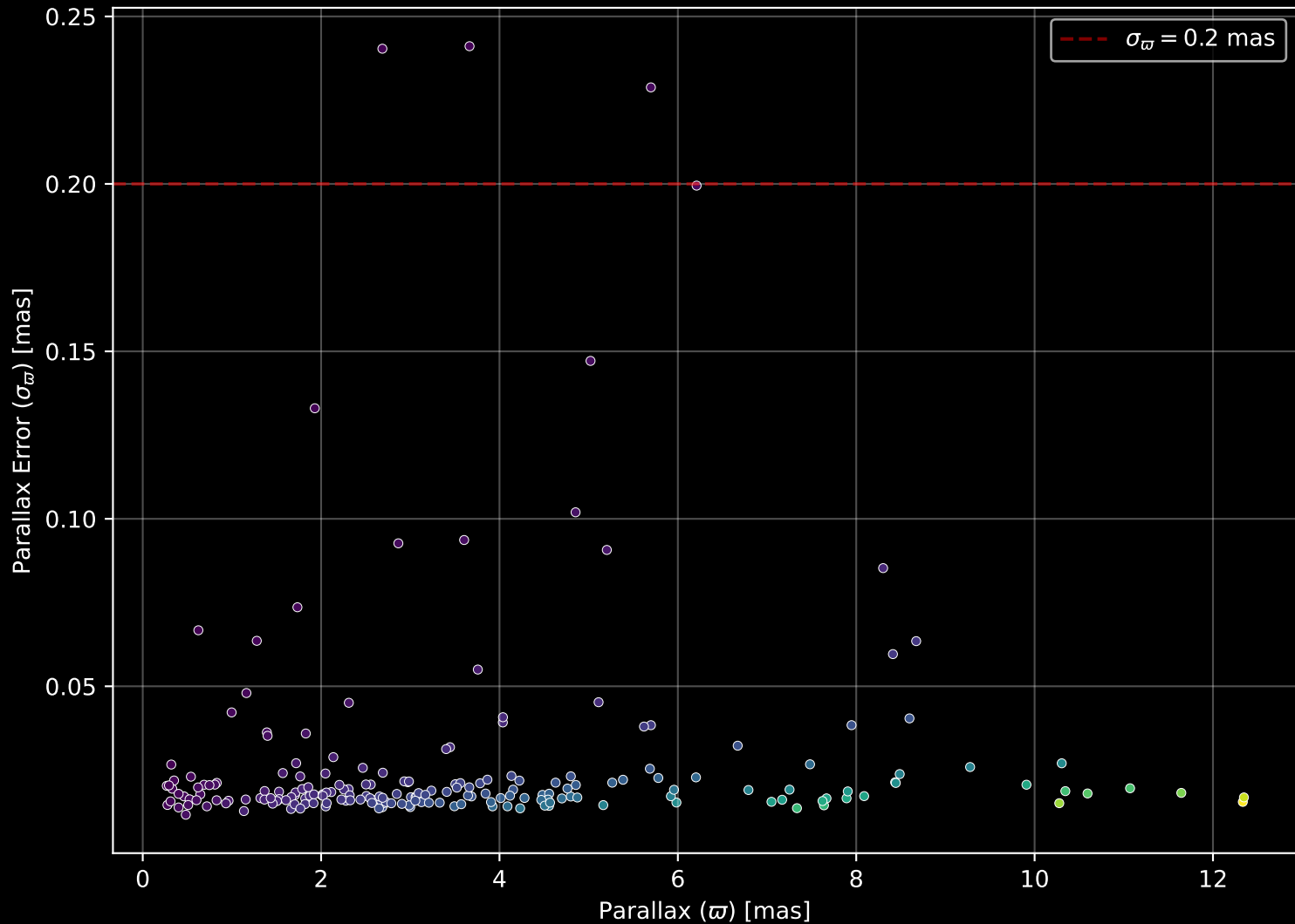
APOGEE DR17 Field: [K2_C12_082-60_btx] Parallax Quality (n= 207)
