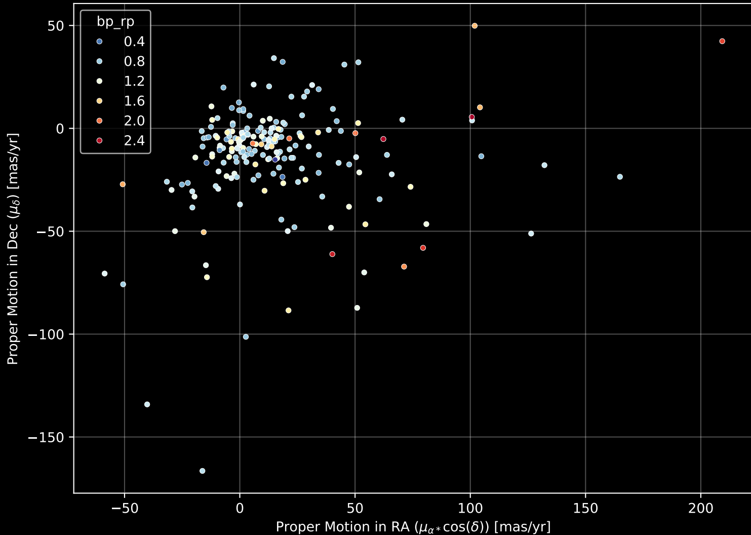
APOGEE DR17 Field: [K2_C12_082-60_btx] Proper Motion Diagram (n= 207)
