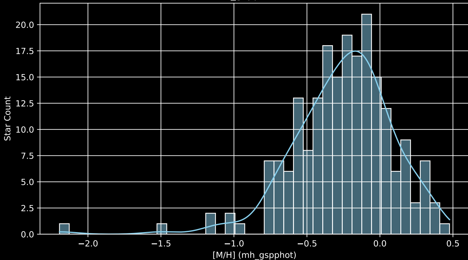
APOGEE DR17 Field: [K2_C12_082-60_btx [M/H] (mh_gspphot) (n= 207)
