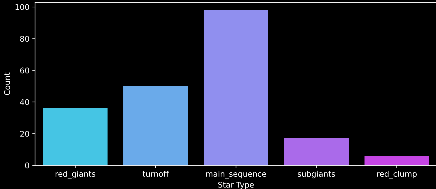
APOGEE DR17 Field: [K2_C12_082-60_btx] Count plot of Star Type
