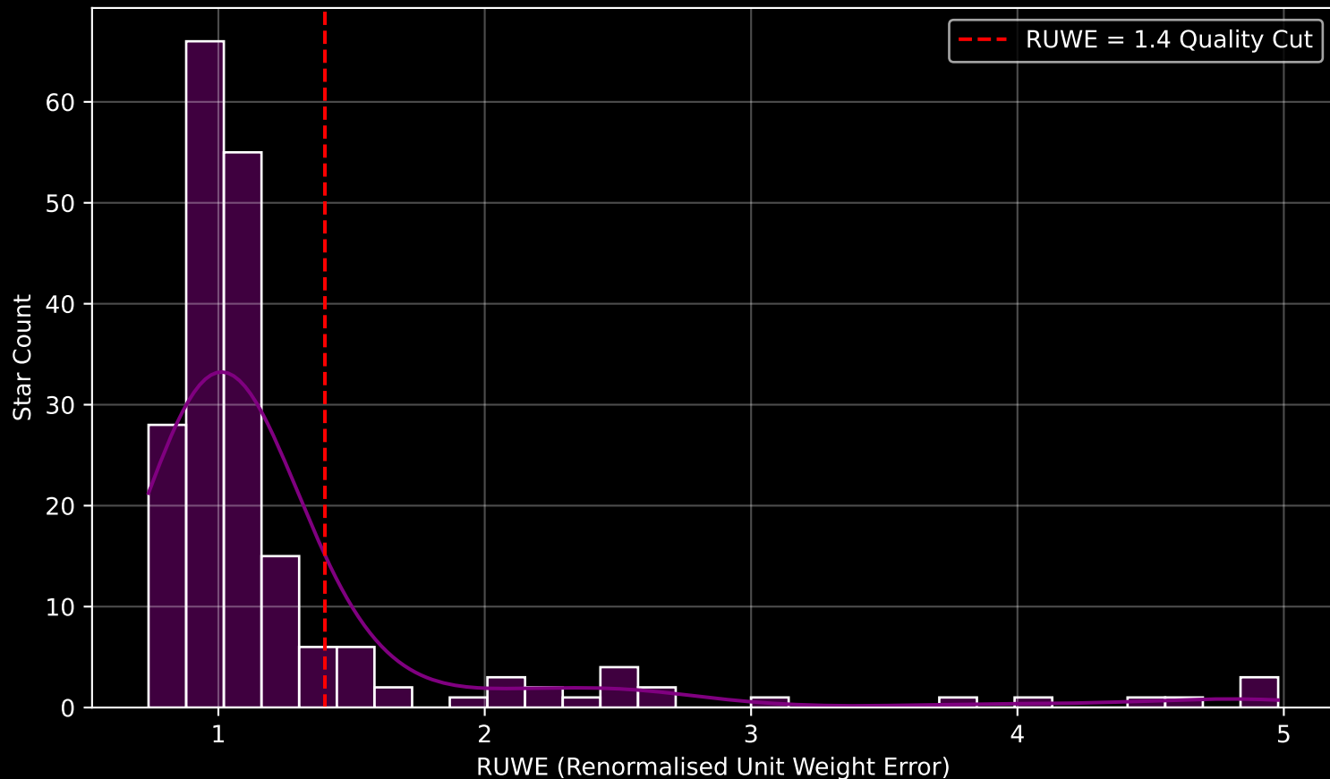
GAPOGEE DR17 Field [K2_C12_082-60_btx] RUWE Distribution (n= 199)
